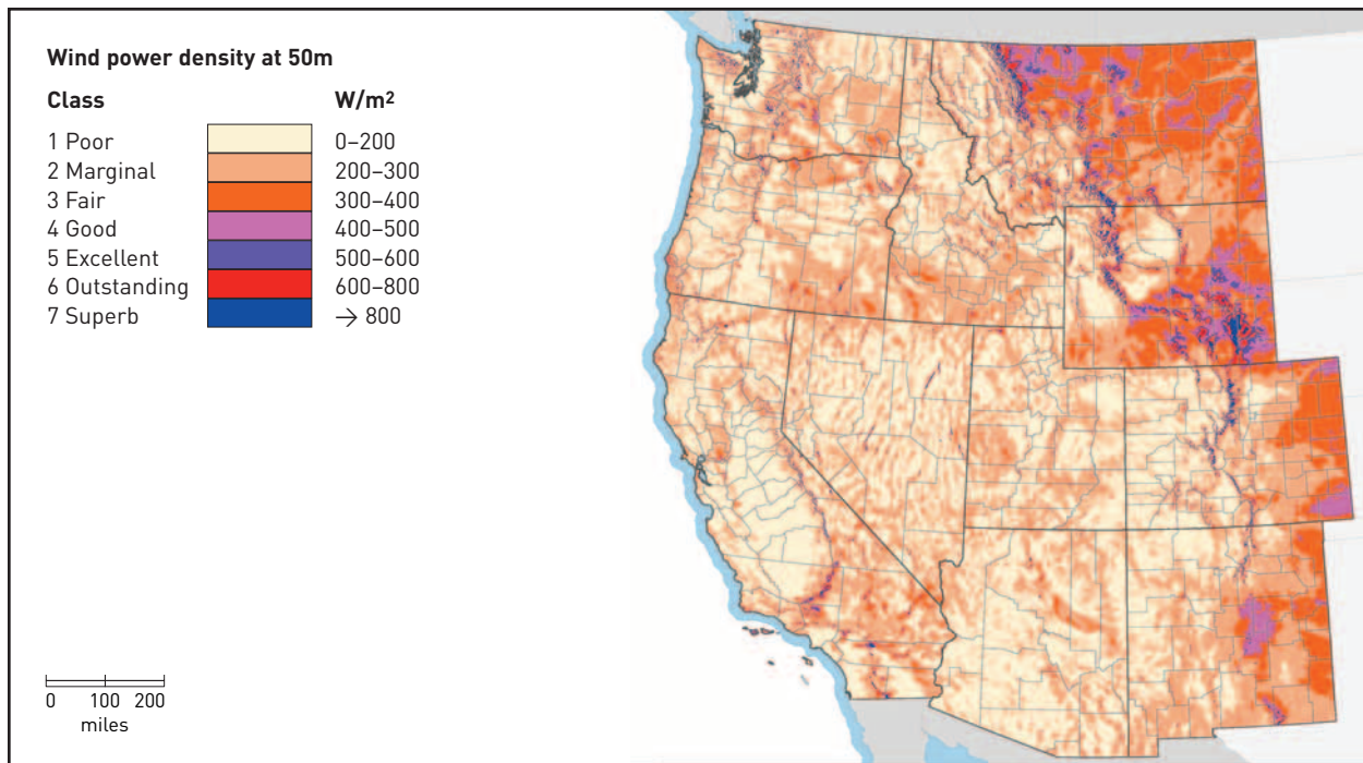
FIGURE 7.1 Wind resources in the western United States
